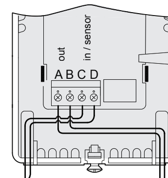
FRONT OF THE BASE
