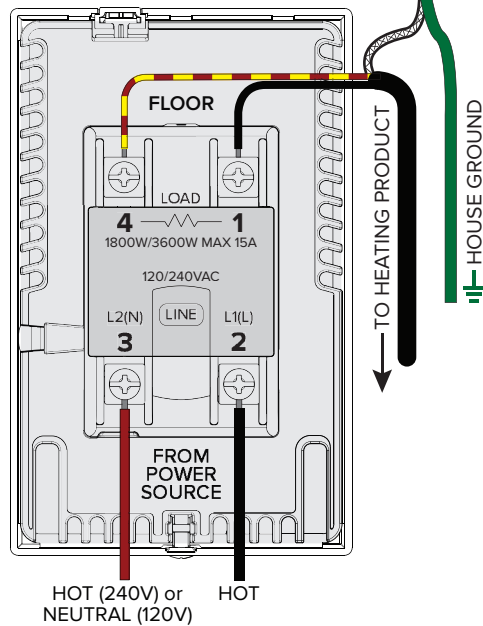
FRONT OF THE THERMOSTAT BASE
