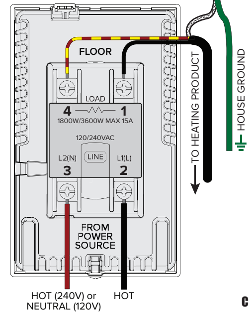
REAR OF THE USG BASE
