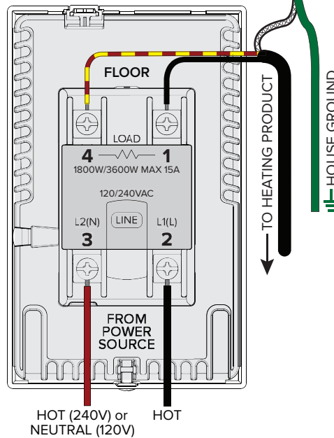
REAR OF THE USG BASE
