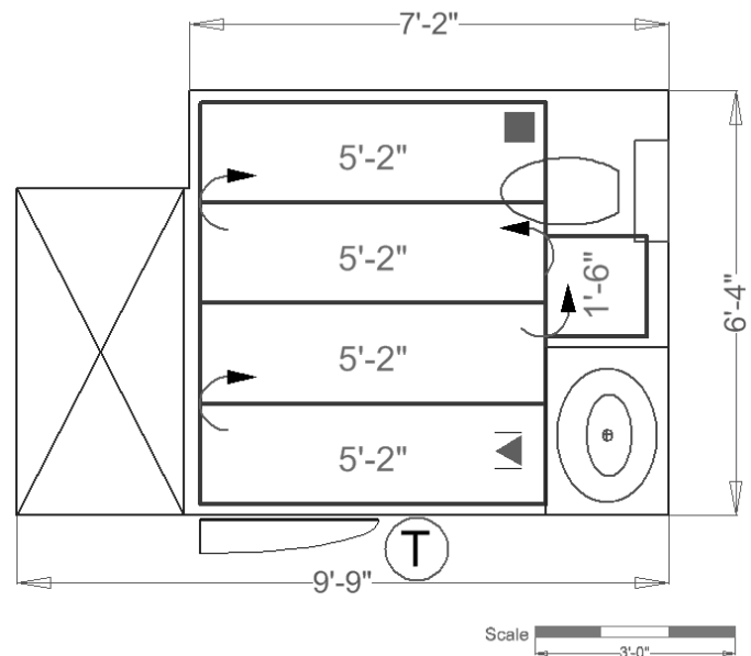
WarmlyYours SmartPlan™ for Bathroom 2
